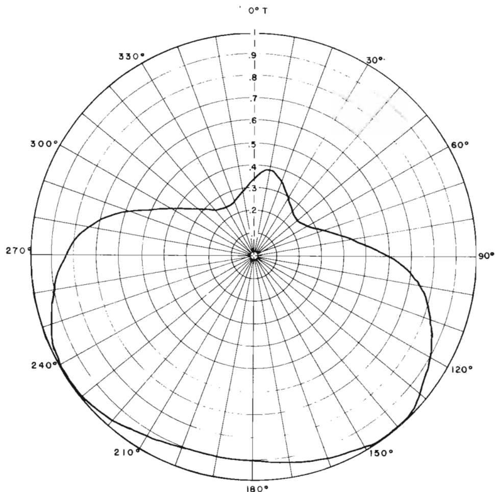
HORIZONTAL PATTERN
